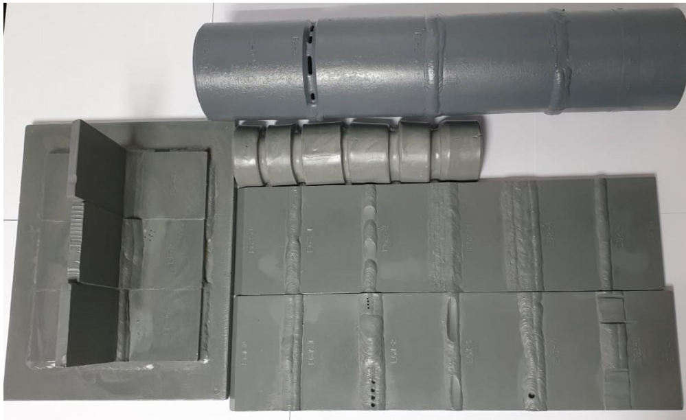
Structural Weld Replica Kit
