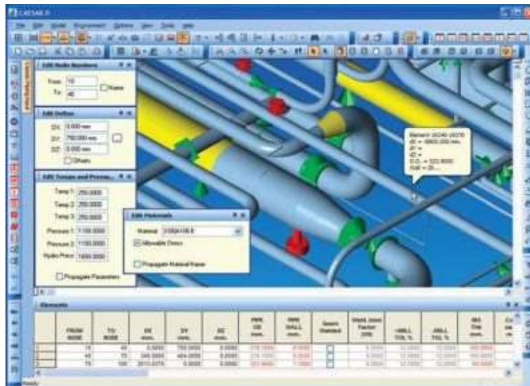
CAESAR II
