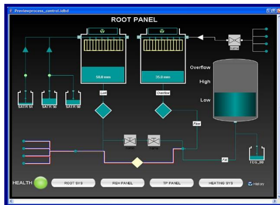
HMI SCADA
