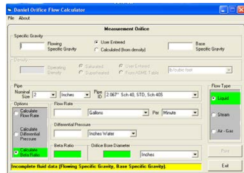
Orifice Flow Calculator Simulator
