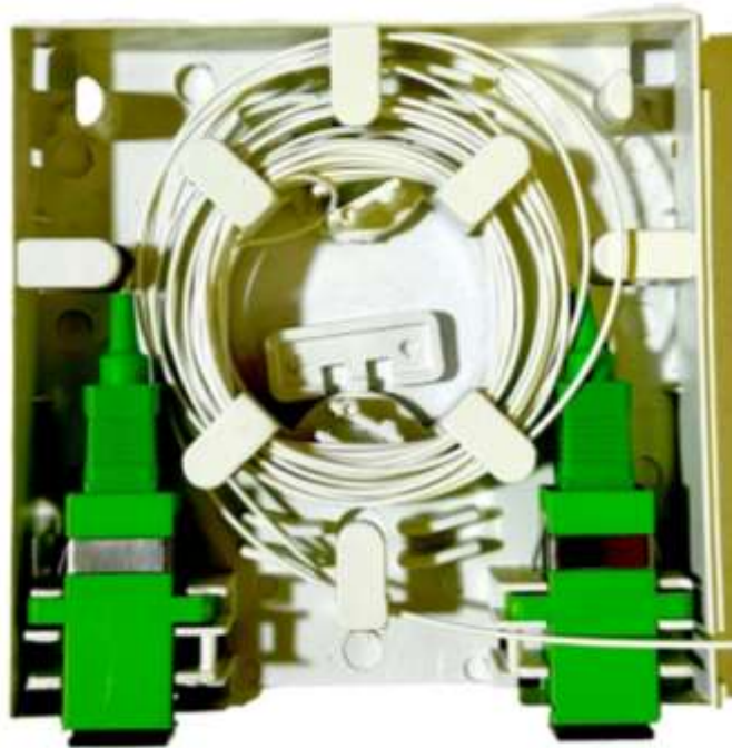
Termination Box with Two Splicing Distribution
